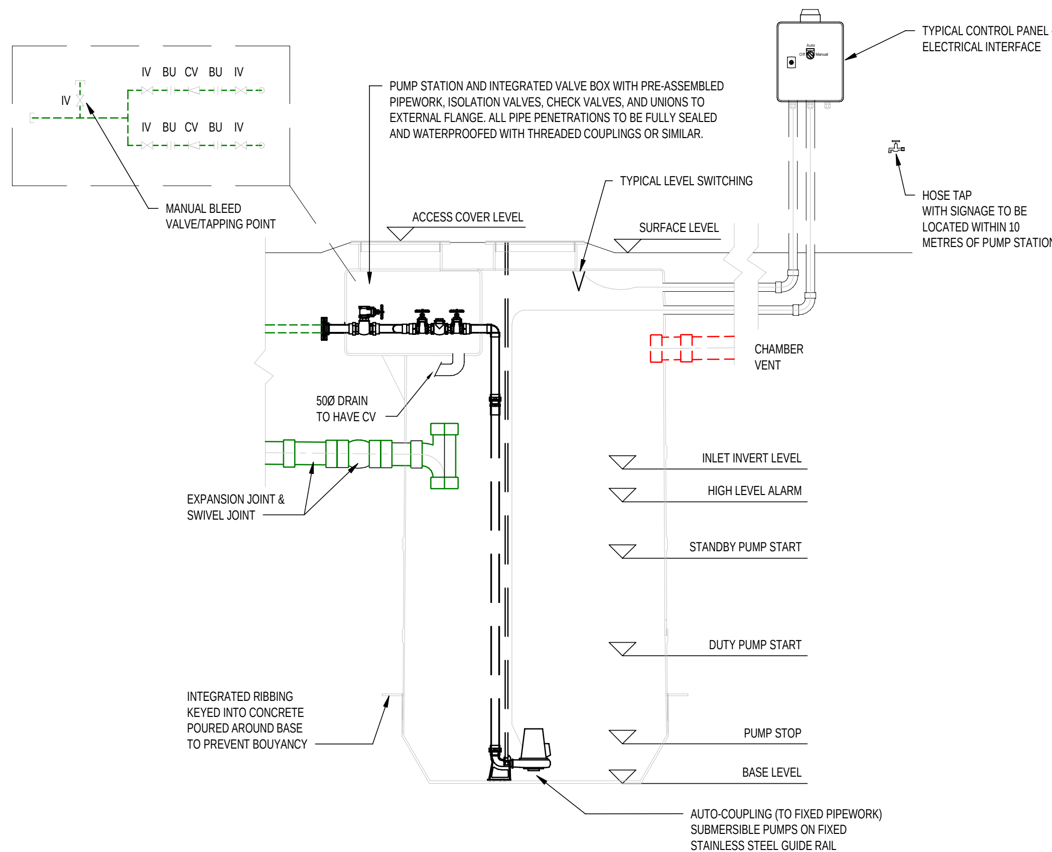
PACKAGED SANITARY DRAINAGE PUMP STATION DETAIL N.T.S.
