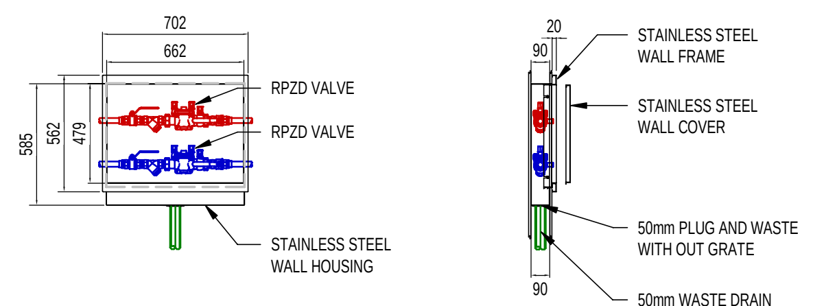
RPZD IN SS WALL BOX DETAIL N.T.S.
