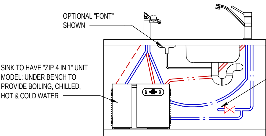
ZIP 4 IN 1 UNDER BENCH MODEL BOILING, CHILLED, HOT & COLD N.T.S.
