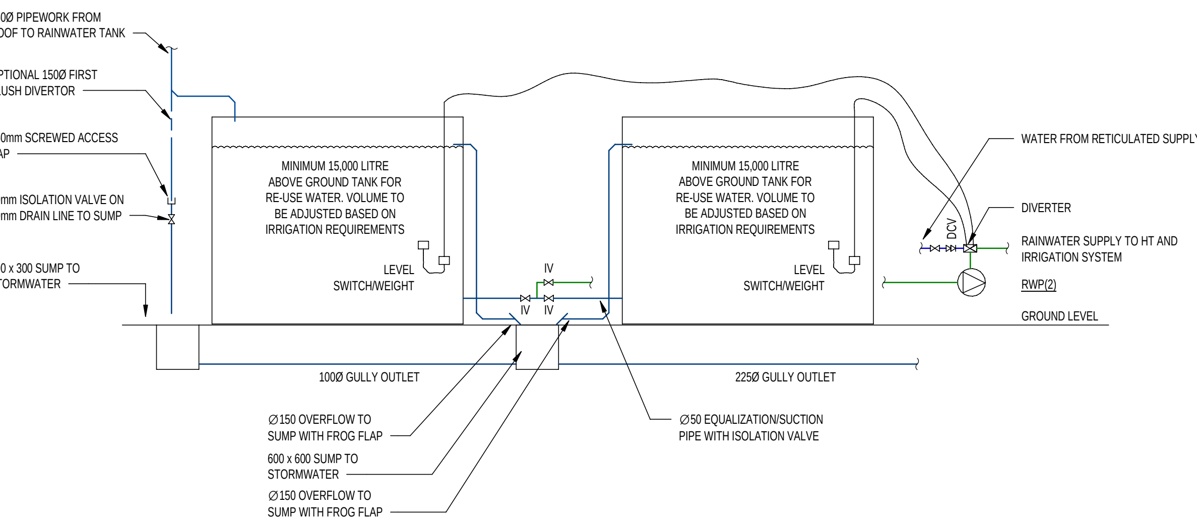
RAINWATER TANK DETAIL - HORTICULTURE BUILDING N.T.S.
