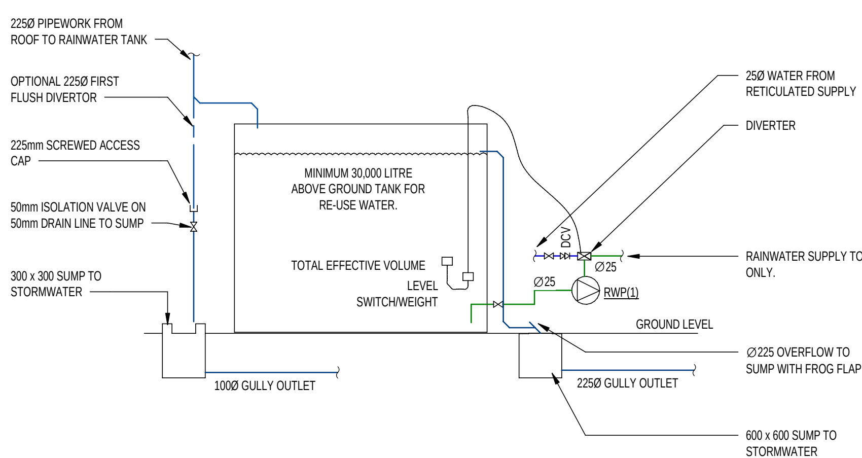
RAINWATER TANK DETAIL - NEW TRADES BUILDING N.T.S.
